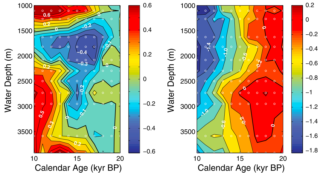
Figure 8. Hovmöller diagrams of benthic \delta^{13}\text{C} and \delta^{18}\text{O} anomalies for the 10–20 kyr B.P. time interval. Anomalies are the stable isotope value at each water depth minus the mean LGM value (19–23 kyr B.P.) at that depth. (left) Benthic \delta^{13}\text{C} anomalies show the mid-depth negative excursion and a concurrent positive anomaly at ~1000 m. The mid-depth negative excursion occurs well before positive anomalies deeper in the water column. (right) Benthic \delta^{18}\text{O} anomalies show the presence of ^{18}\text{O} -enriched water mass below 2500 m from the LGM to ~15 kyr B.P.
