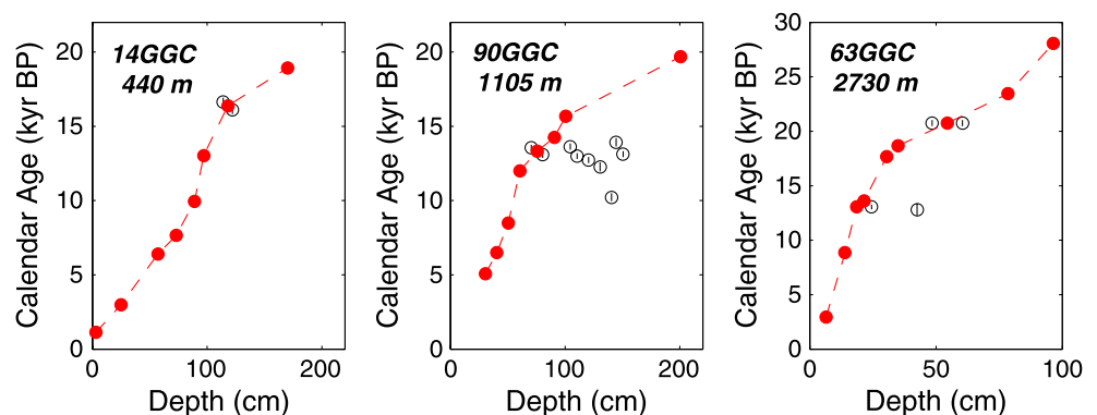
Figure 2. Calendar ages (red circles) and age models (dashed lines) for cores KNR159-5-14GGC, KNR159-5-90GGC, and KNR159-5-63GGC based on G. ruber (>250 \mu\text{m} ). The error bars for each calendar age represent the \pm 1\sigma uncertainty. In most cases, the error bar is smaller than the symbol. Age reversals not included in each age model are shown as black circles. In the case of 14GGC, the two ages near 120 cm were averaged to create one control point. Cores 90GGC and to a lesser extent 63GGC have ages out of stratigraphic order. A similar phenomenon occurs in other Brazil Margin cores and is related to deep burrowing [Sortor and Lund, 2011; Hoffman and Lund, 2012] and the variable abundance of planktonic and benthic foraminifera (see Figure 3). Note that the benthic stable isotopic time series for cores 14GGC, 90GGC, and 63GGC lack obvious evidence of bioturbation from up section (Figure 4).
