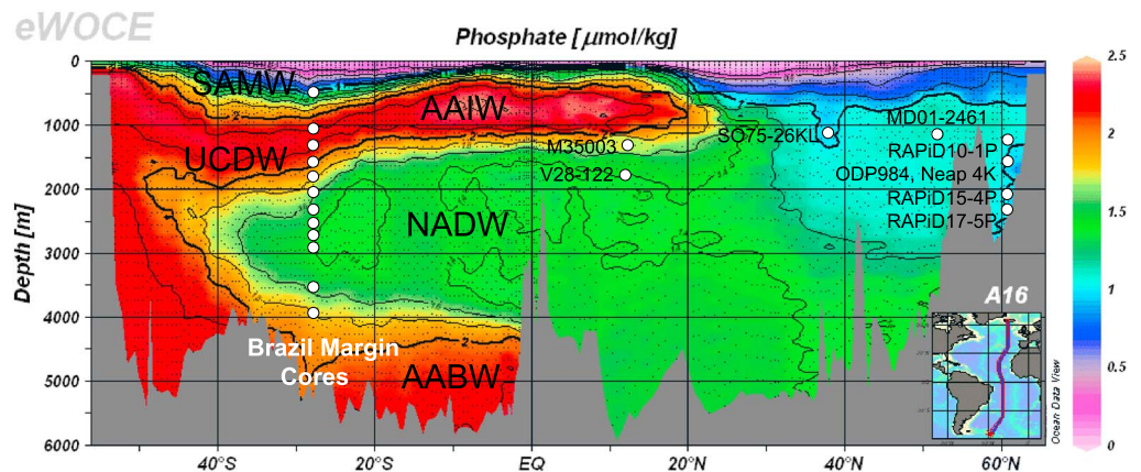
Figure 1. Locations of the 12 cores used in this paper (Table 1) superimposed on the phosphate concentration of the World Ocean Circulation Experiment A16 section in the Atlantic Ocean [Schlitzer, 2000]. The Brazil Margin cores at 27°S span Antarctic Intermediate Water (AAIW), Upper Circumpolar Deep Water (UCDW), and North Atlantic Deep Water (NADW). Also shown are the approximate core locations for NEAP 4K [Rickaby and Elderfield, 2005], ODP984 [Praetorius et al., 2008], RAPiD 10-1P, RAPiD 15-4P and RAPiD 17-5P [Thornalley et al., 2010], SO75-26KL [Zahn et al., 1997], M35003 [Zahn and Stuber, 2002], V28-122 [Yu et al., 2010], and MD01-2461 [Peck et al., 2006].
